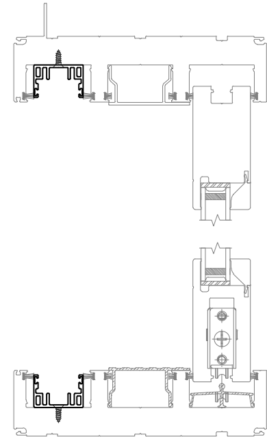
VERTICAL SECTION
