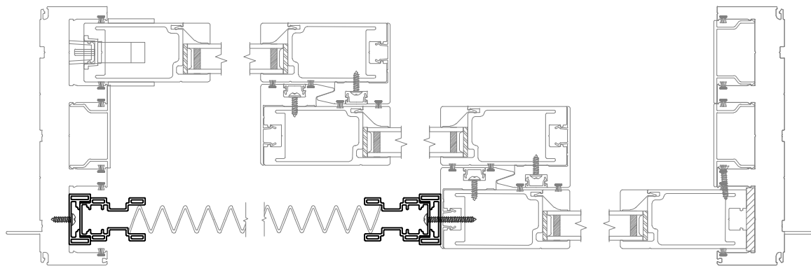
HORIZONTAL SECTION
