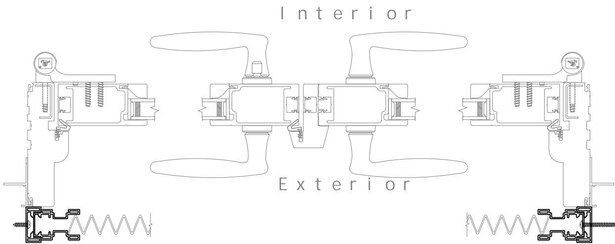
HORIZONTAL SECTION
