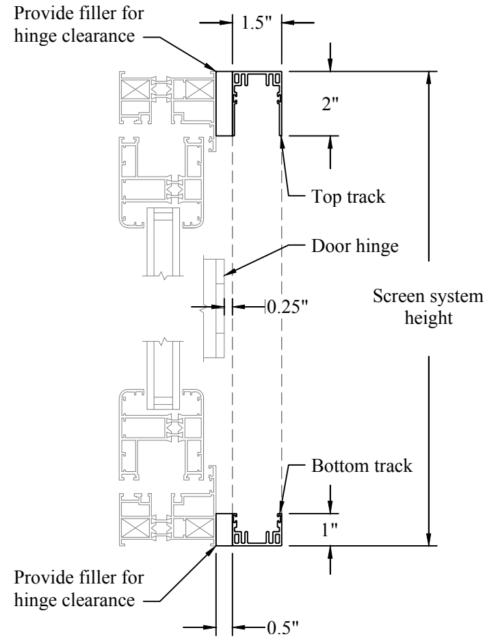
NON-FLUSH TRANSITION
