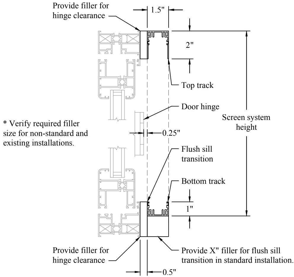
FLUSH TRANSITION
